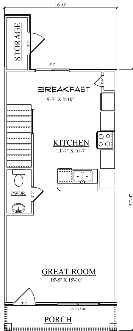
1ST FLOOR LAYOUT
